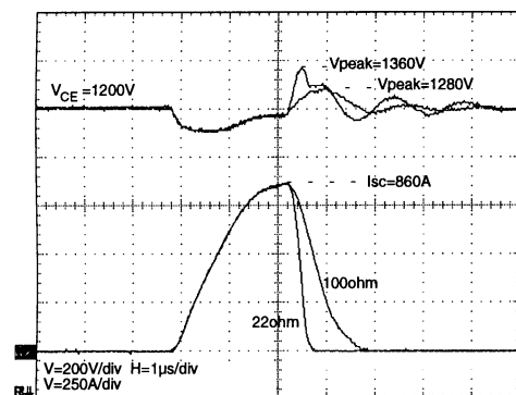
Fig.14 Effect of R_{\text{goff-SC}} in short - circuit
