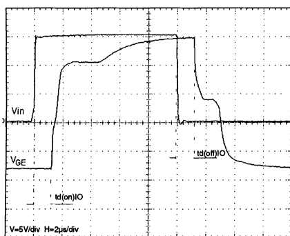
Fig. 11 Input and output voltage propagation time
