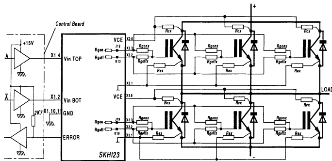
Fig. 10 Preferred circuit for paralleld dual IGBT-modules
