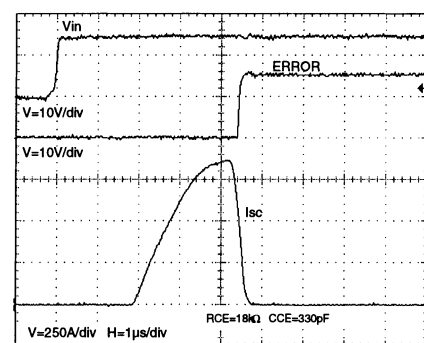
Fig.13 Short circuit and ERROR propagation time worste case ( V_{IN} with SC already present)
